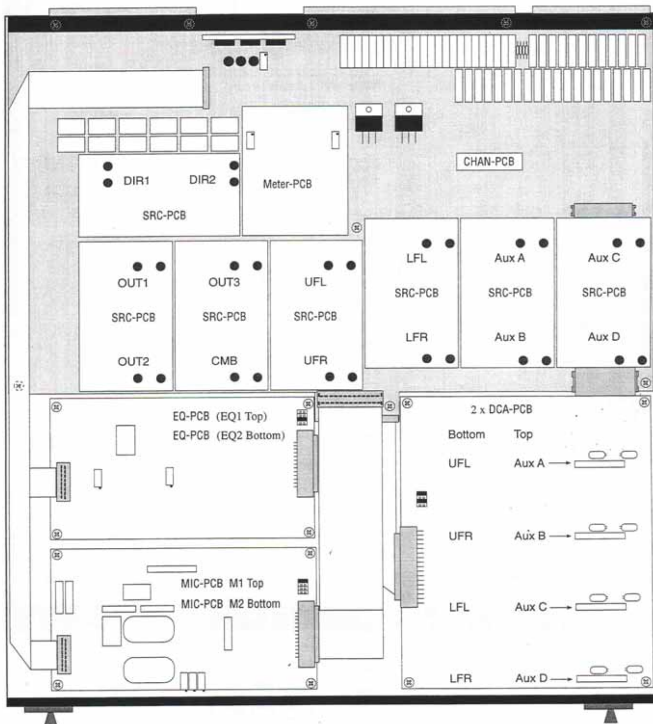
Figure 3.9 - Audio Channel - Top View
